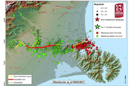
Epicenters and aftershocks of 2010-11 New Zealand earthquakes.
